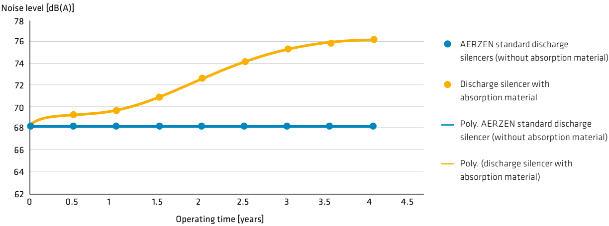
Noise development due to wear of the absorbent in the discharge silencer Pipe sound level at constant volume flow 30 m³/min at 600 mbar (g)
